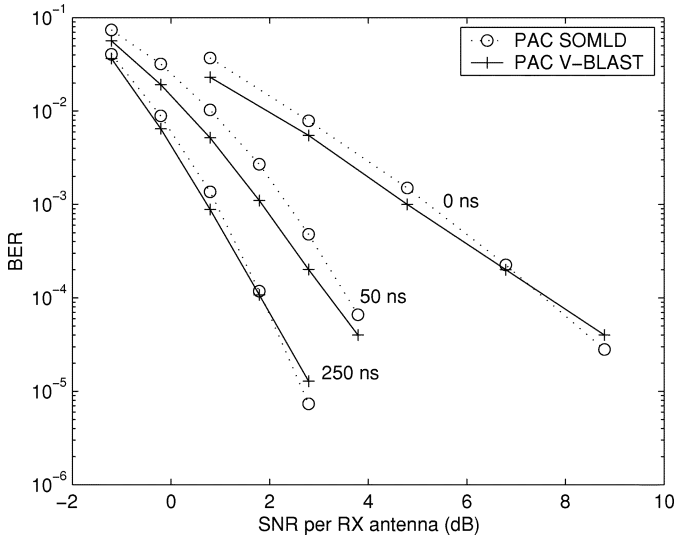
Fig. 6. BER performance for 4 \times 4 PAC schemes, BPSK, rate 1/2 coding, and frequency-selective Rayleigh fading with an exponentially decaying PDP with different rms delay spreads.
